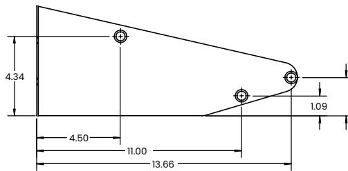
ROD POSITIONS, DISPLAY BRACKET 1 REMOVED FOR CLARITY
