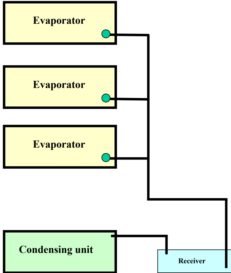
Liquid Line Feed to Stacked Evaporator Coils
