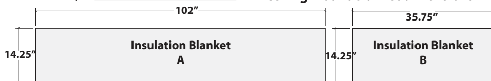
Ceiling Mount blanket dimensions
