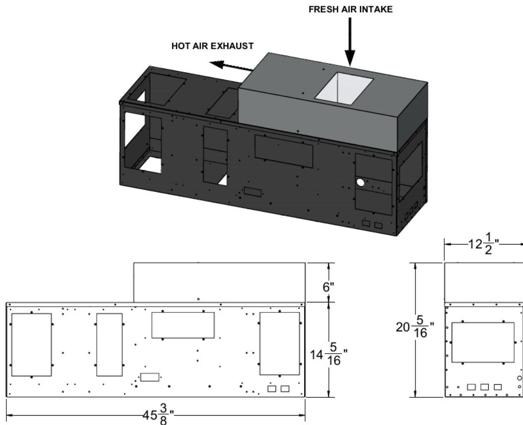
3400H SOUND HOOD DIMENSIONAL DRAWING
